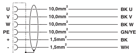
Contact assignment of M40 plugs/sockets
